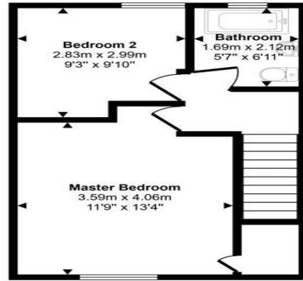
First Floor Approx 34 sq m / 363 sq ft
