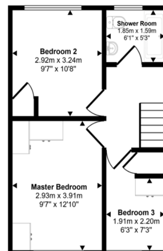
First Floor Approx 36 sq m / 390 sq ft
