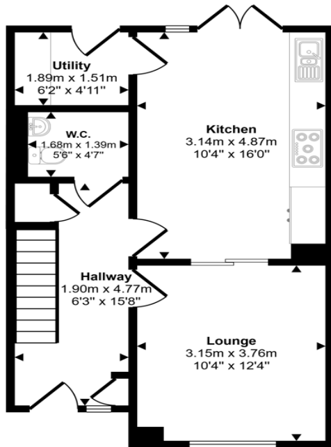
Ground Floor Approx 44 sq m / 472 sq ft
