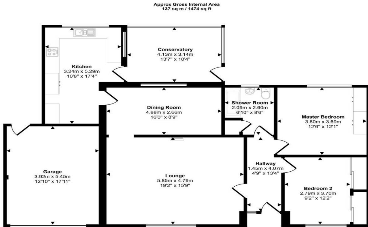
Floorplan
