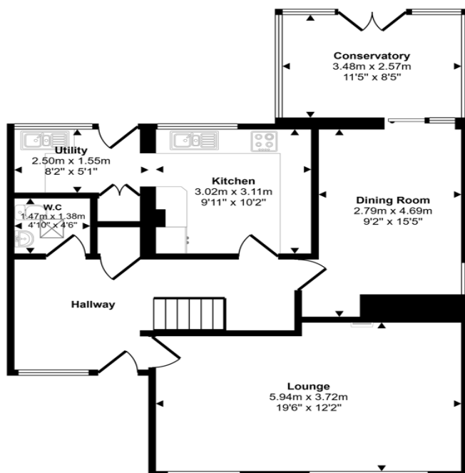
Ground Floor Approx 77 sq m / 827 sq ft
