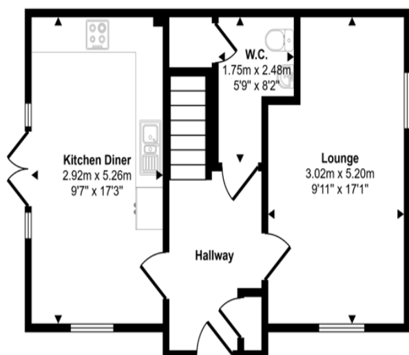
Ground Floor Approx 45 sq m / 479 sq ft
