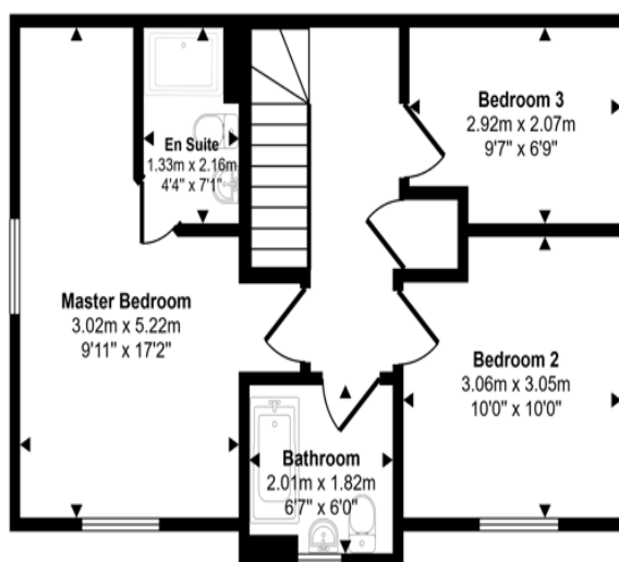
First Floor Approx 45 sq m / 482 sq ft
