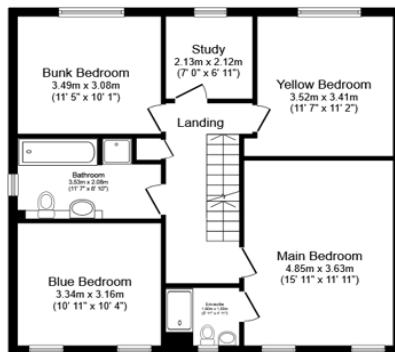
First Floor Floor area 77.2 m 2 (831 sq.ft.)
