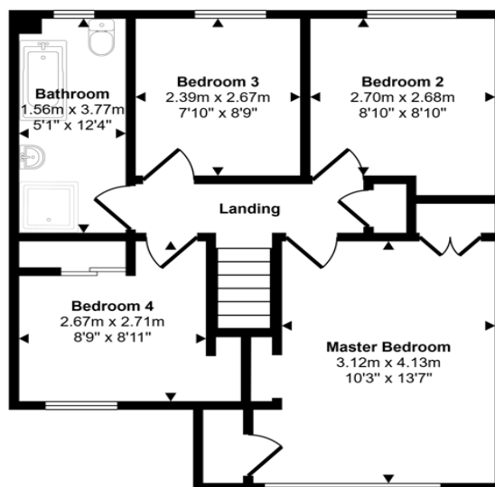
First Floor Approx 52 sq m / 557 sq ft
